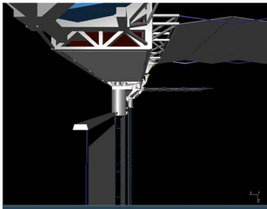
Figure 2.4-5: S3 lower truss, +Y, orbital sunrise (left), and orbital noon (right).
