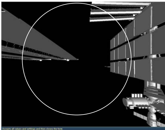
Figure 2.4-4: S3 lower truss, -X, orbital noon (left), and orbital sunrise (right).
